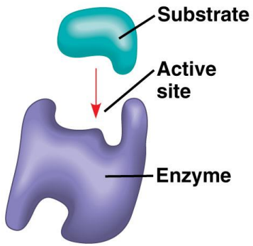
(a) Normal binding
