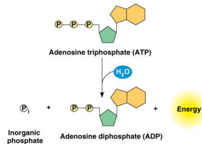
(b) The hydrolysis of ATP
