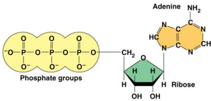
(a) The structure of ATP
