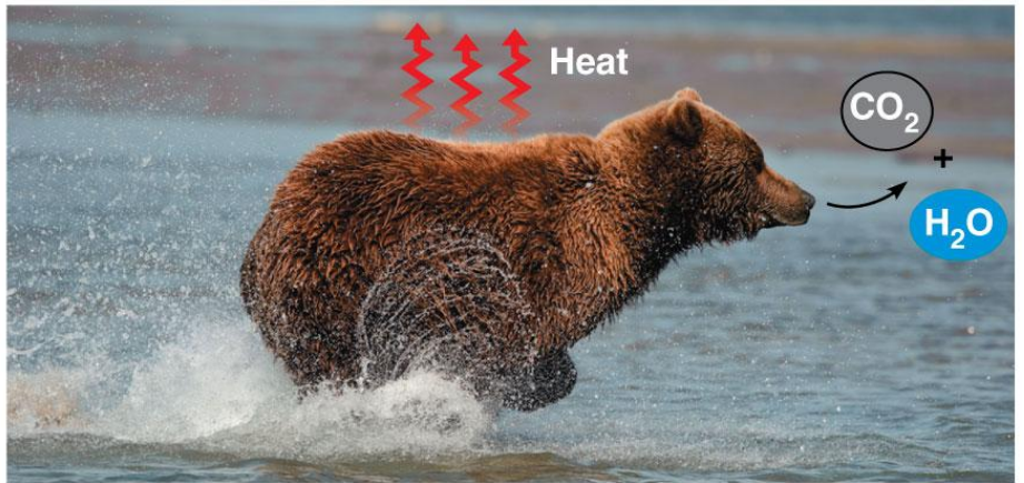
(b) Second law of thermodynamics
