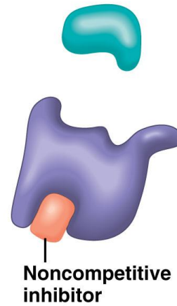
(c) Noncompetitive inhibition
