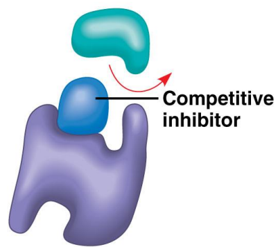
(b) Competitive inhibition
